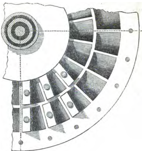
Plan (one-fourth) of the fixed part, showing the Guide Curves and six of the Sluces or Regulators.
